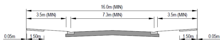
Figure 6.3: Access Street (16m) Cross Section 11
