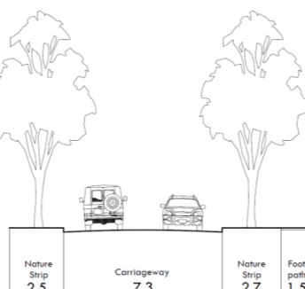
Figure 6.4: Access Lane (14m) Cross Section
