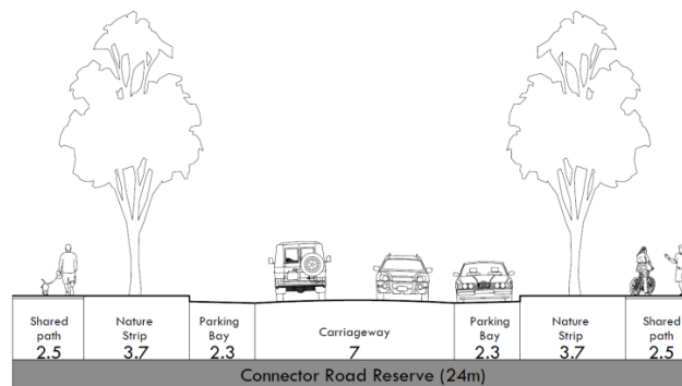
Figure 6.2: Connector Street (24m) Cross Section
